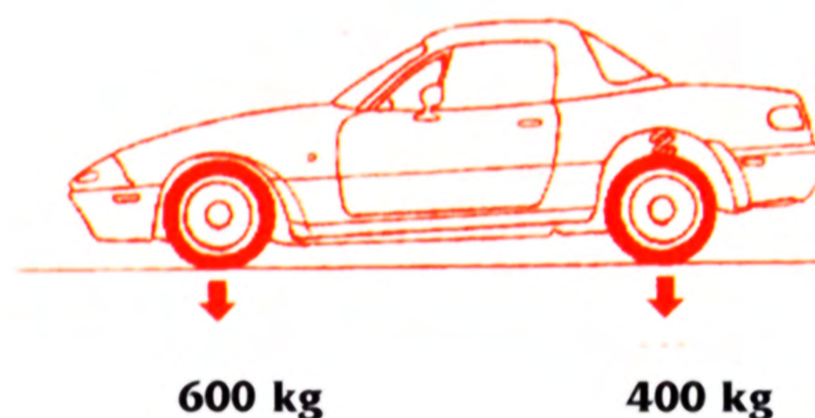
Weight transfer to front during braking.
